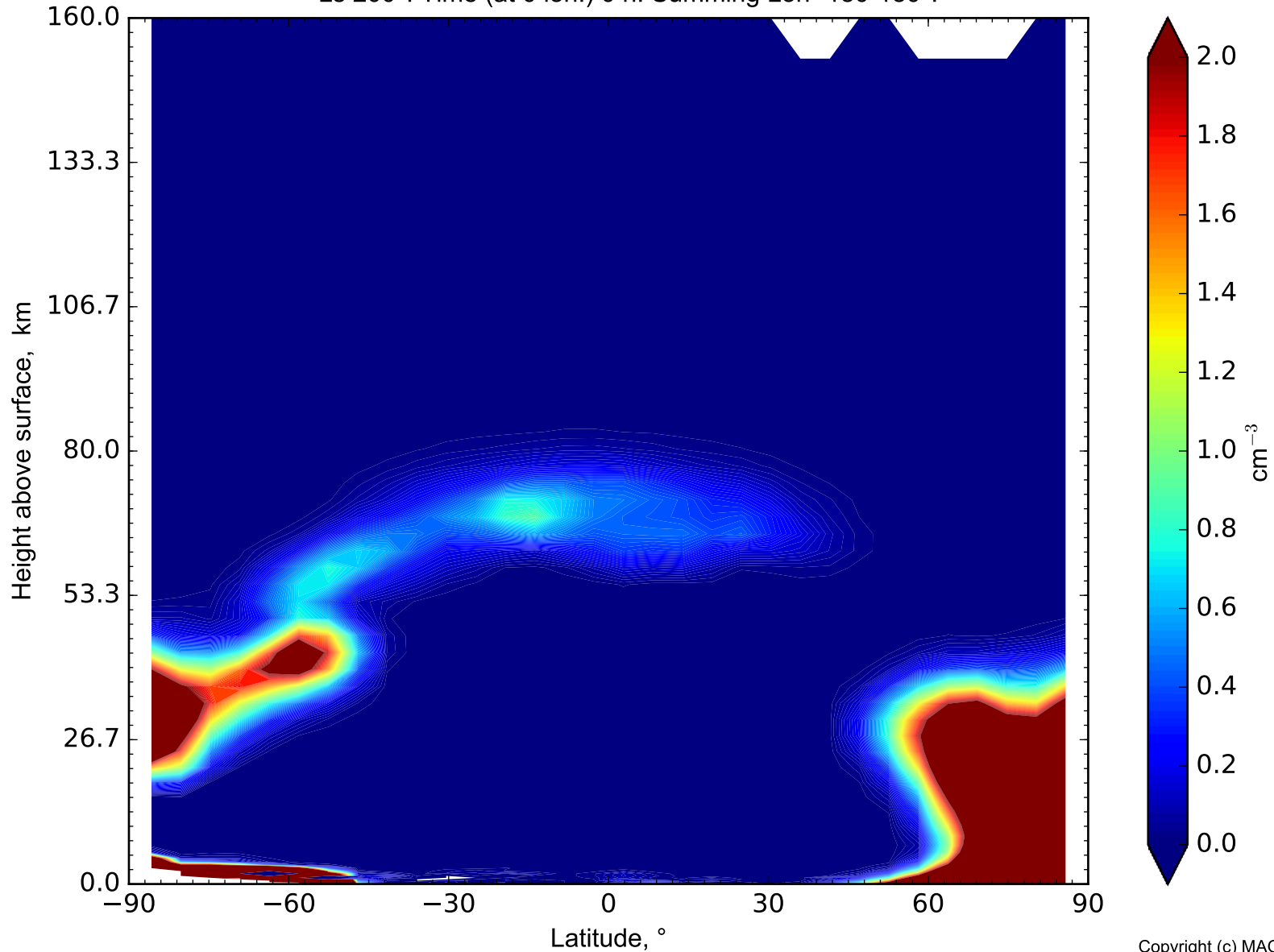
H 2 O ice number density on Mars Ls 200°. Time (at 0 lon.) 0 h. Summing Lon -180-180°.
