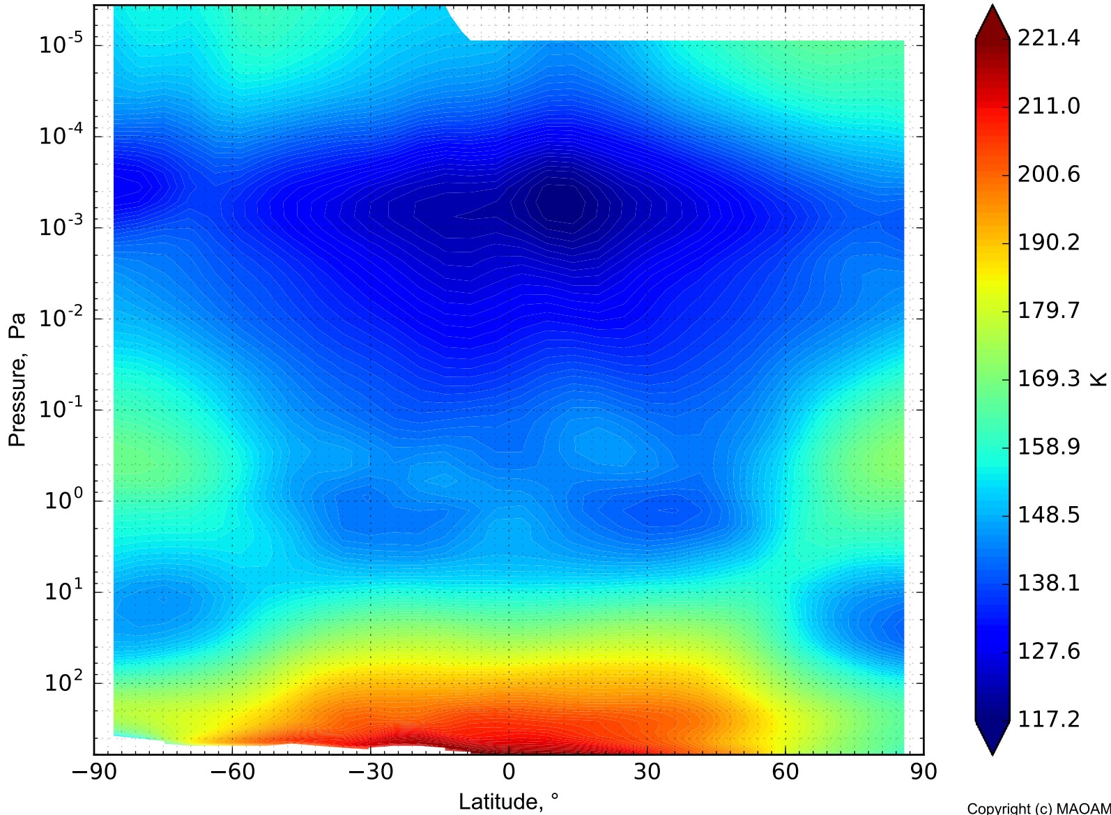
Temperature on Mars Diurnally averaged. Average Ls 355-360°. Lon -180°.
