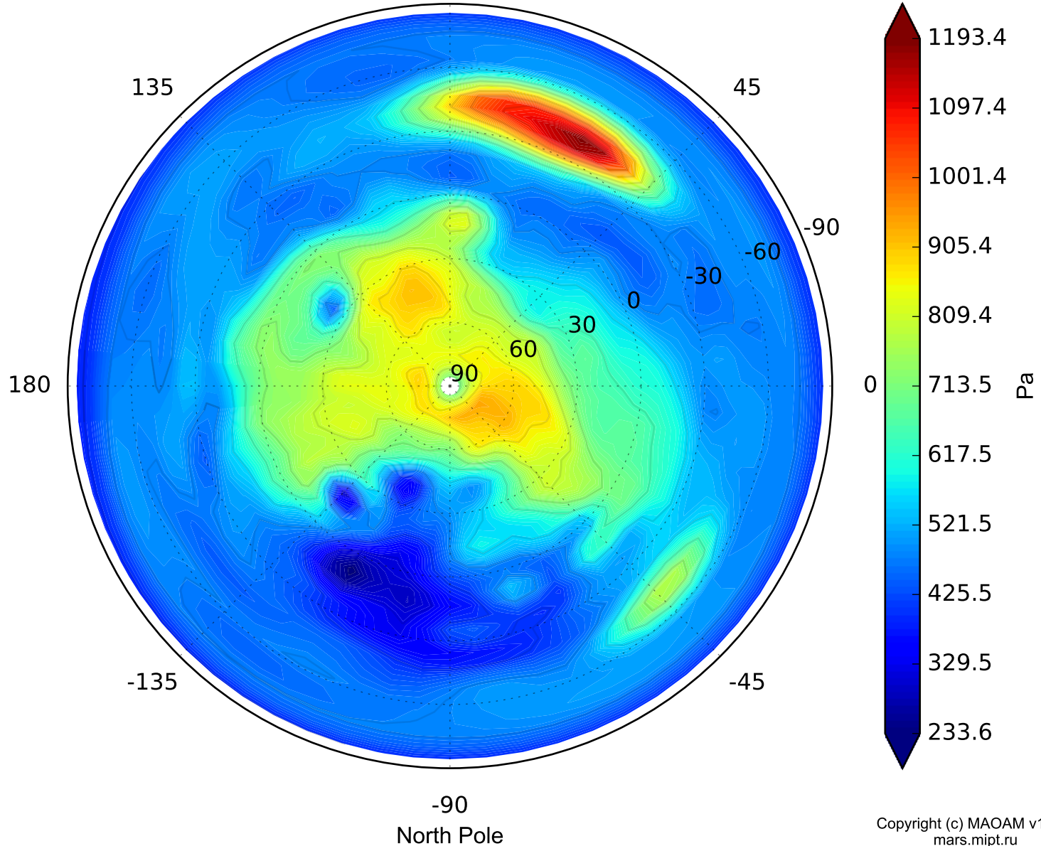
Surface pressure on Mars Diurnally averaged. Average Ls 0-360°. Pre 607 Pa.
