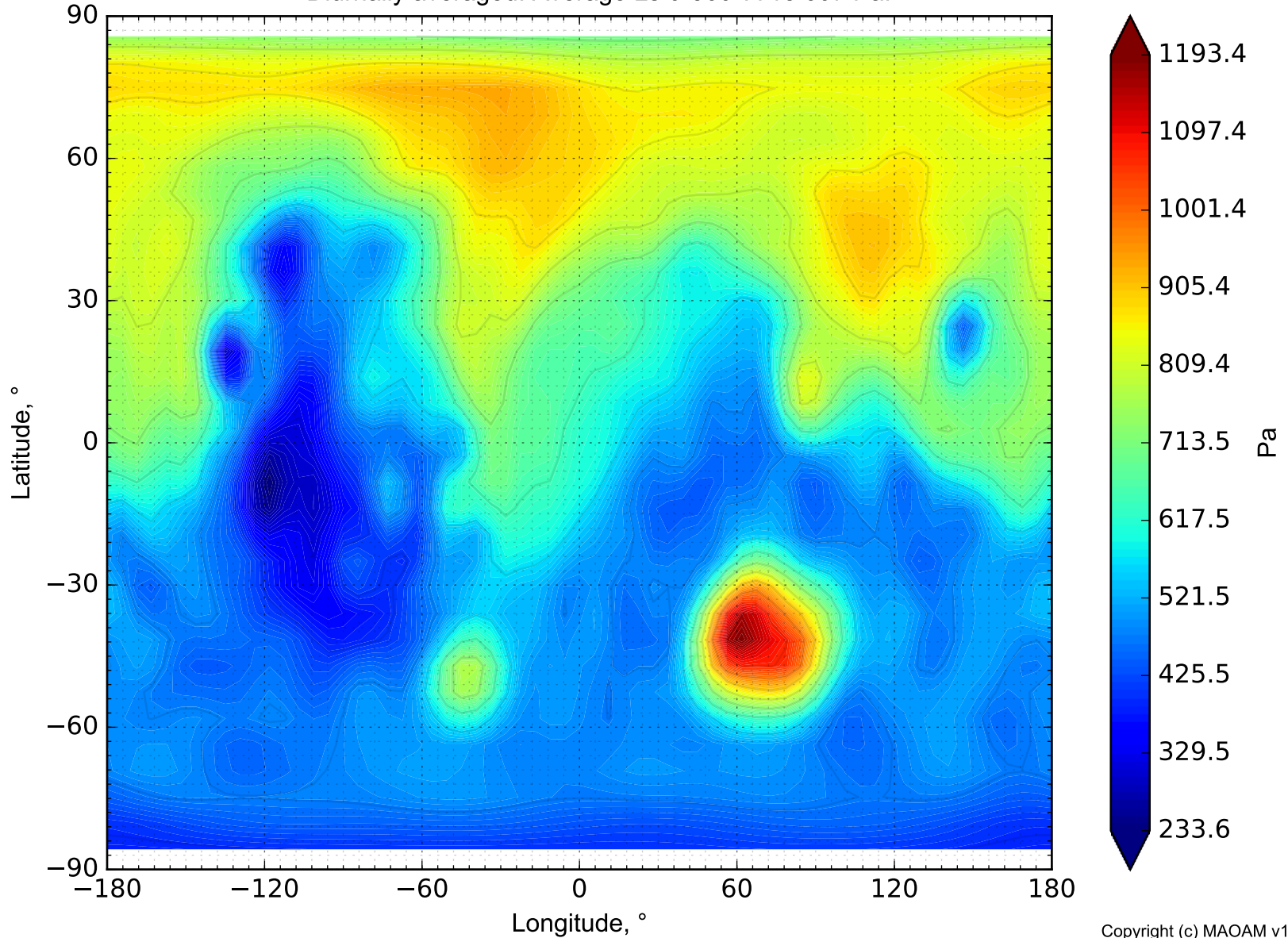
Surface pressure on Mars Diurnally averaged. Average Ls 0-360°. Pre 607 Pa.
