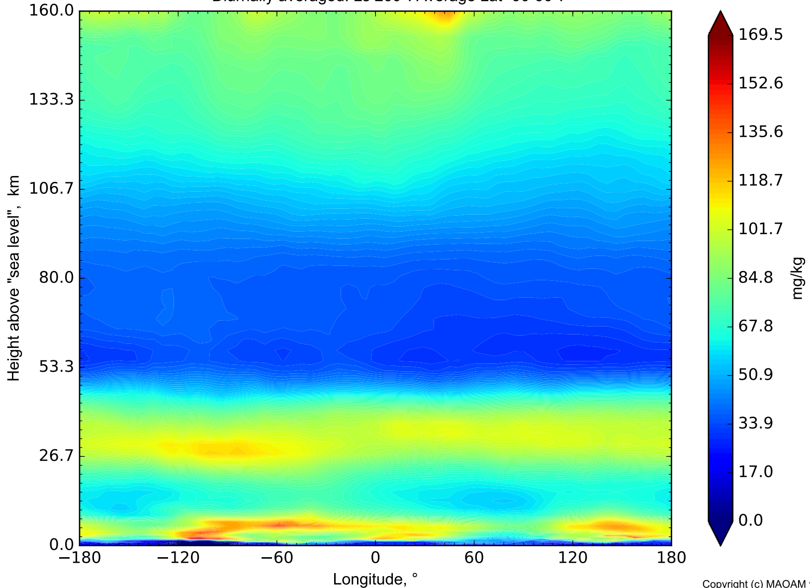
H 2 O vapor mix. ratio on Mars Diurnally averaged. Ls 260°. Average Lat -90-90°.
