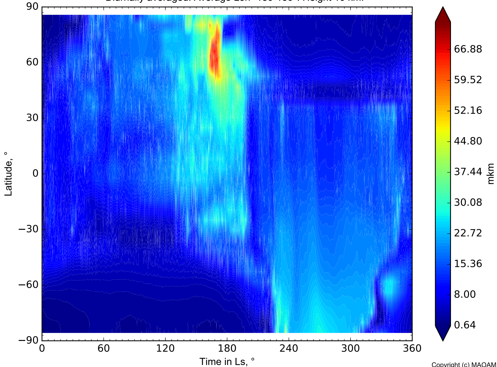
H 2 O ice particle radius on Mars Diurnally averaged. Average Lon -180-180°. Height 10 km.
