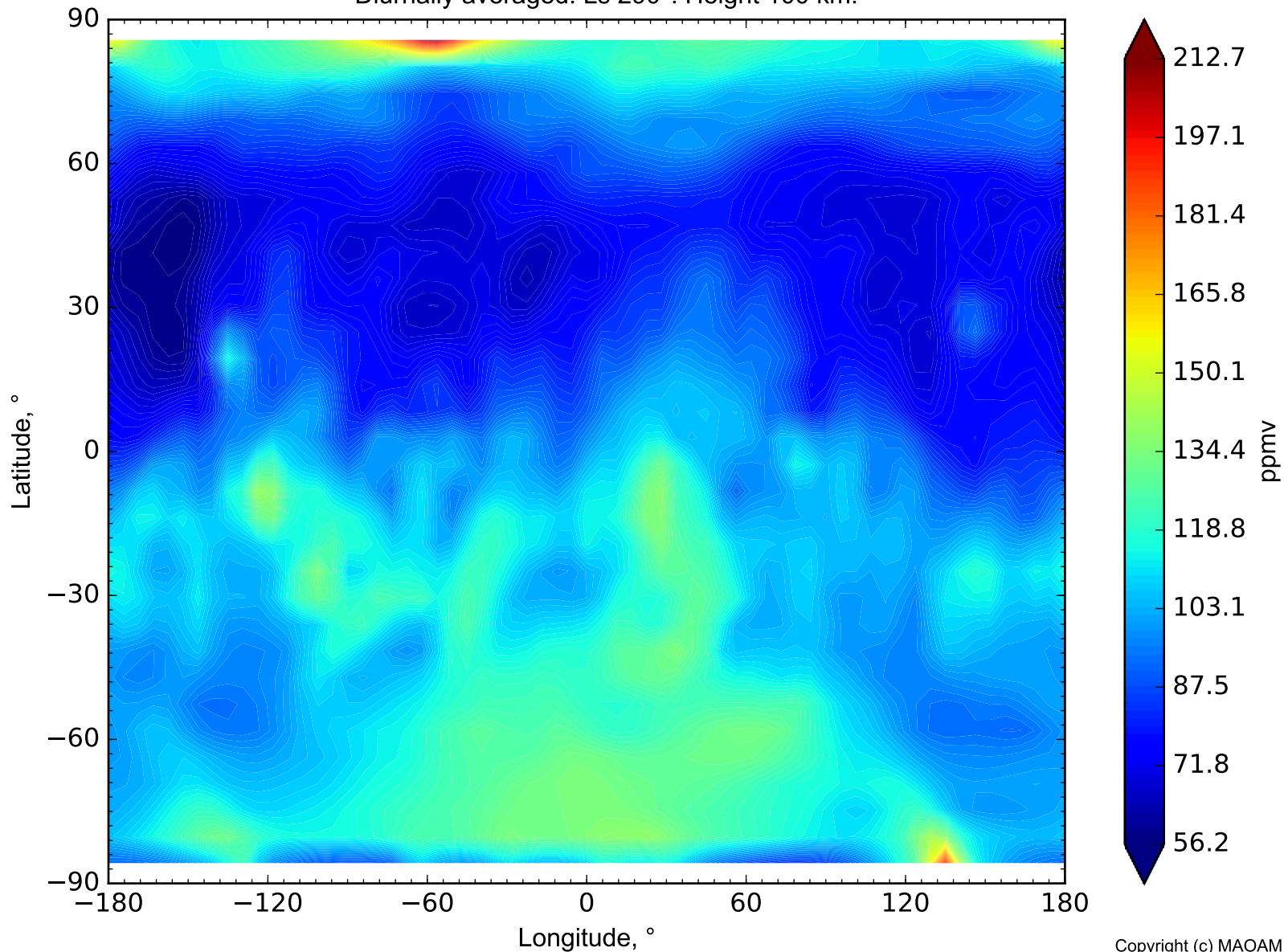
H 2 O vapor mix. ratio on Mars Diurnally averaged. Ls 290°. Height 100 km.
