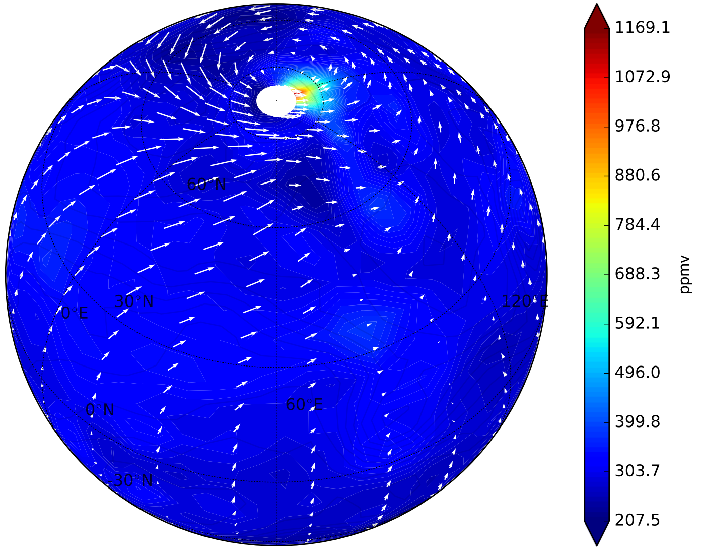
H 2 O vapor mix. ratio on Mars Ls 210°. Time (at 0 lon.) 15 h. Average Height 0-160 km.
