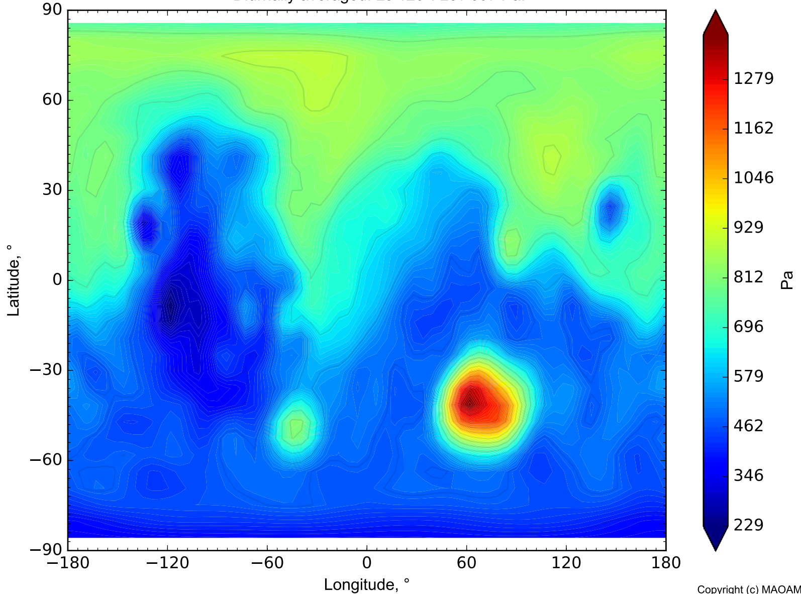
Surface pressure on Mars Diurnally averaged. Ls 120°. Lev 607 Pa.
