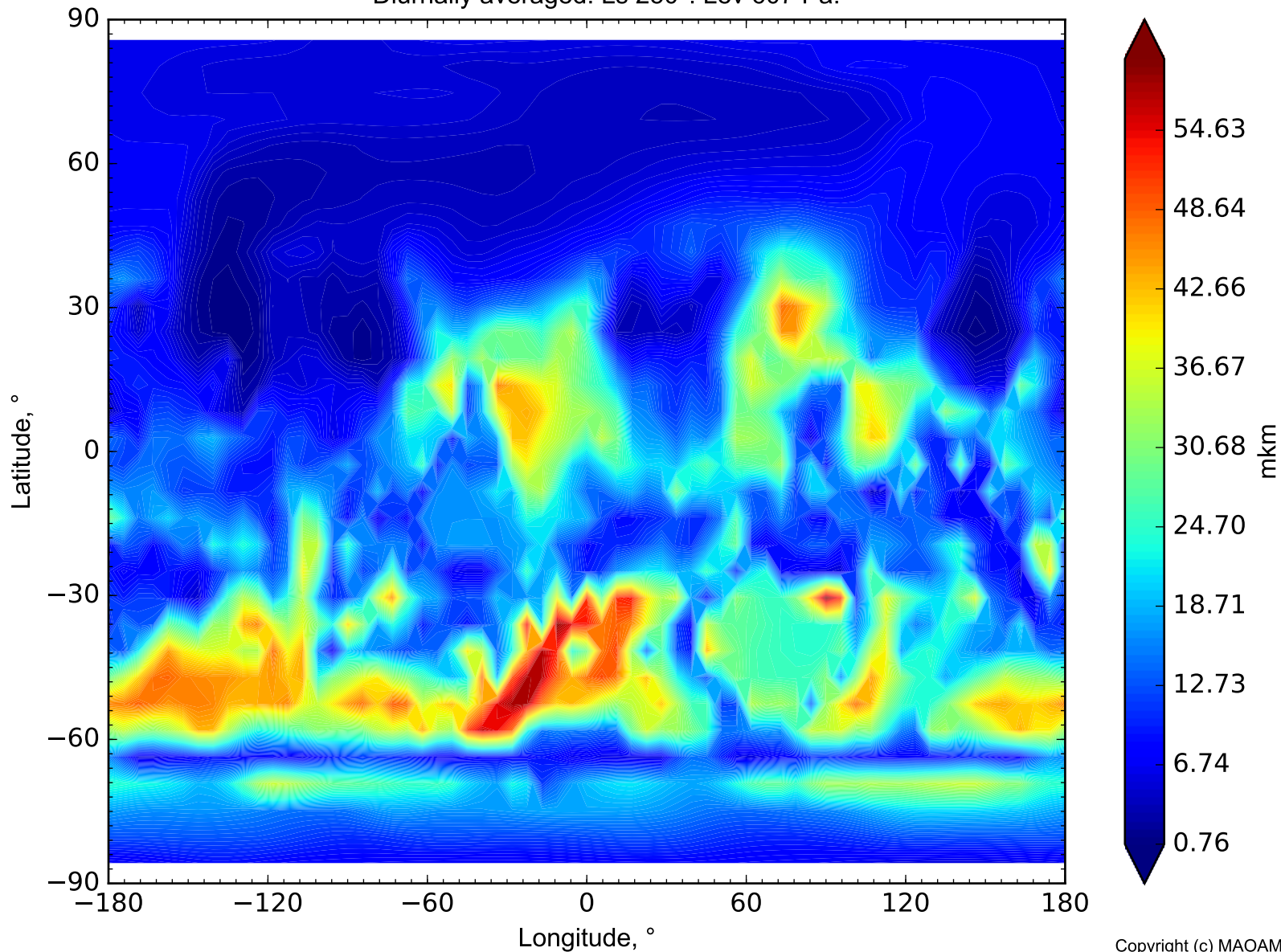
H 2 O ice particle radius on Mars Diurnally averaged. Ls 250°. Lev 607 Pa.
