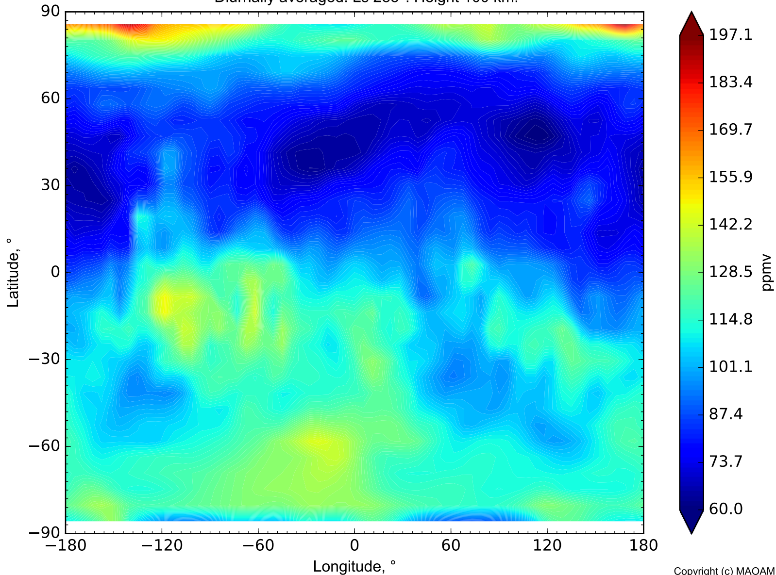
H 2 O vapor mix. ratio on Mars Diurnally averaged. Ls 285°. Height 100 km.
