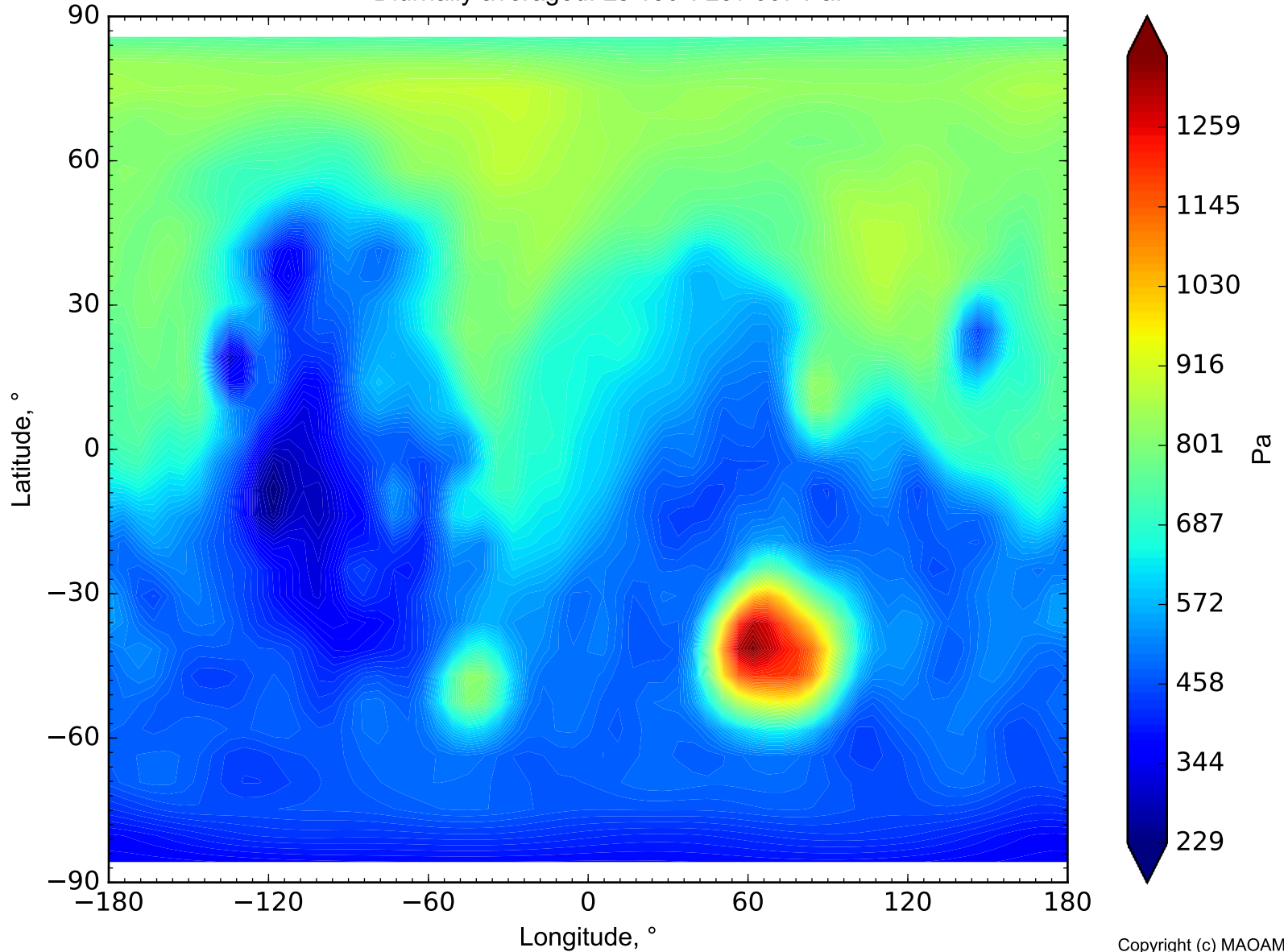
Pressure on Mars Diurnally averaged. Ls 130°. Lev 607 Pa.
