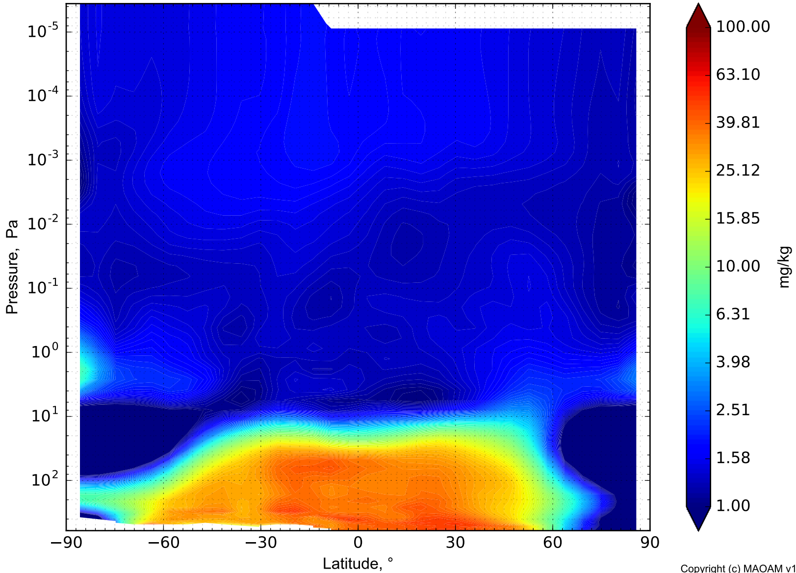
H 2 O vapor mix. ratio on Mars Diurnally averaged. Average Ls 355-360°. Lon -180°.
