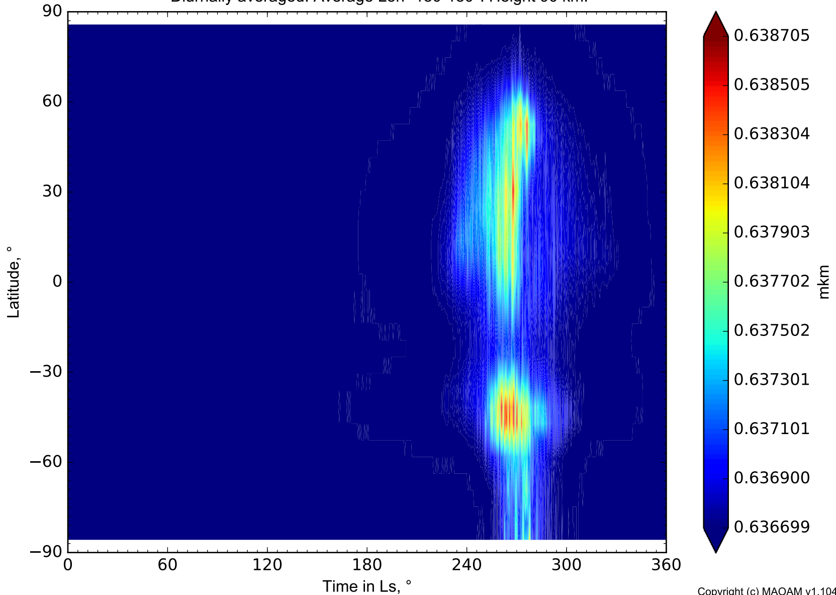
H 2 O ice particle radius on Mars Diurnally averaged. Average Lon -180-180°. Height 90 km.
