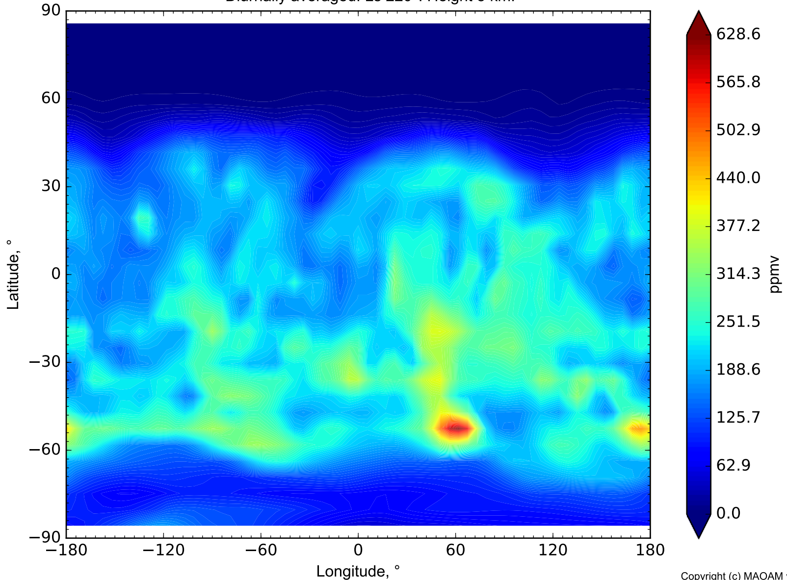
H 2 O vapor mix. ratio on Mars Diurnally averaged. Ls 220°. Height 5 km.
