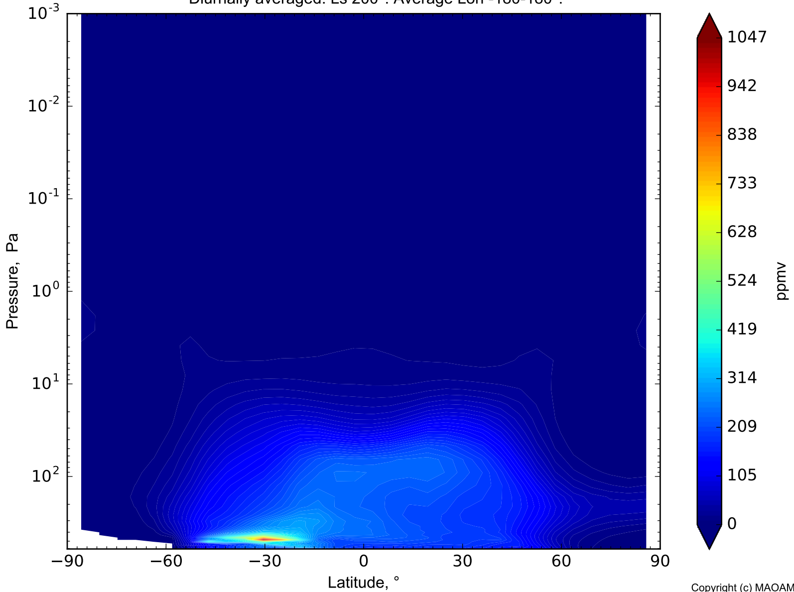
H 2 O vapor mix. ratio on Mars Diurnally averaged. Ls 200°. Average Lon -180-180°.
