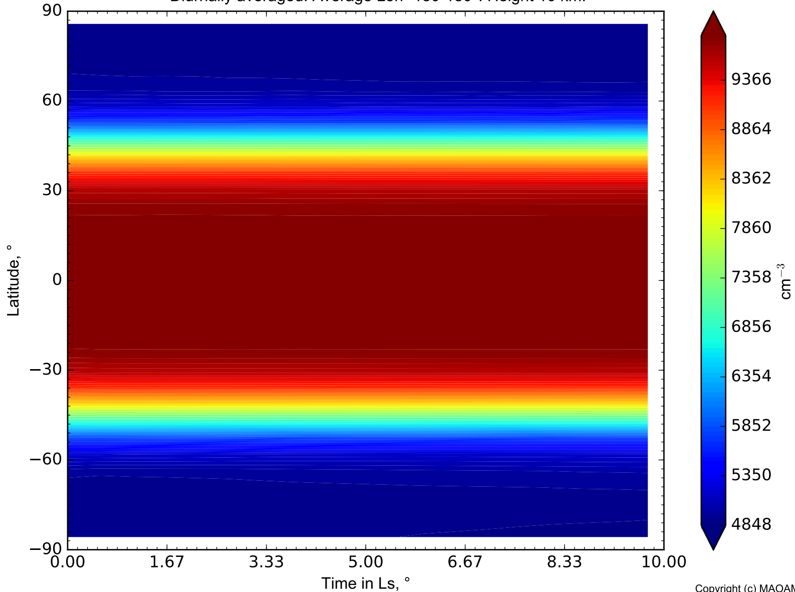
Dust number density (given) on Mars Diurnally averaged. Average Lon -180-180°. Height 10 km.
