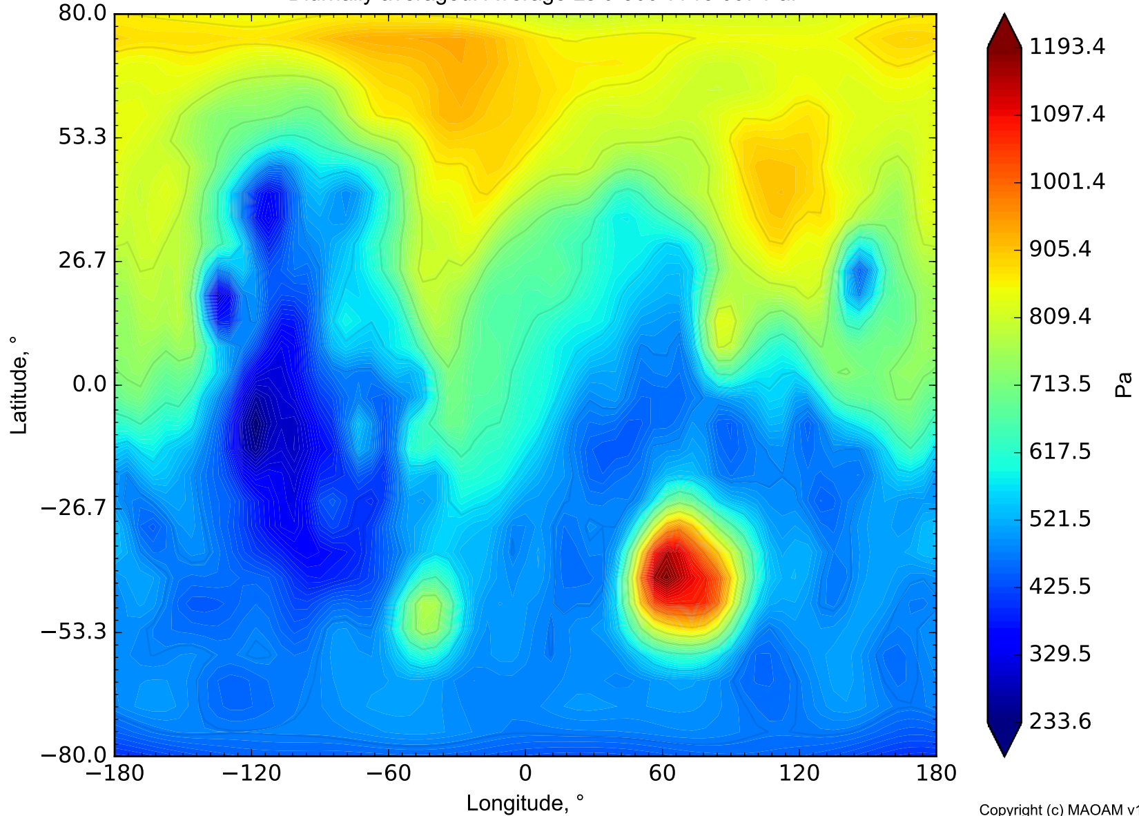
Surface pressure on Mars Diurnally averaged. Average Ls 0-360°. Pre 607 Pa.
