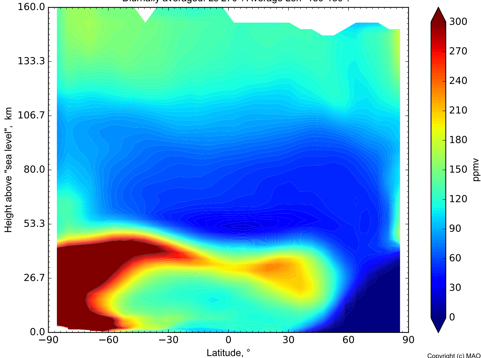
H 2 O vapor mix. ratio on Mars Diurnally averaged. Ls 270°. Average Lon -180-180°.
